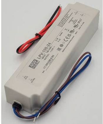
860-0001-011 24 VDC 100-WATT, 90-264 VAC POWER SUPPLY
