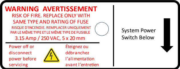
301-5091-001 EVO SYS. WARNING/FUSE/POWER SWITCH LABEL, UNIVERSAL
